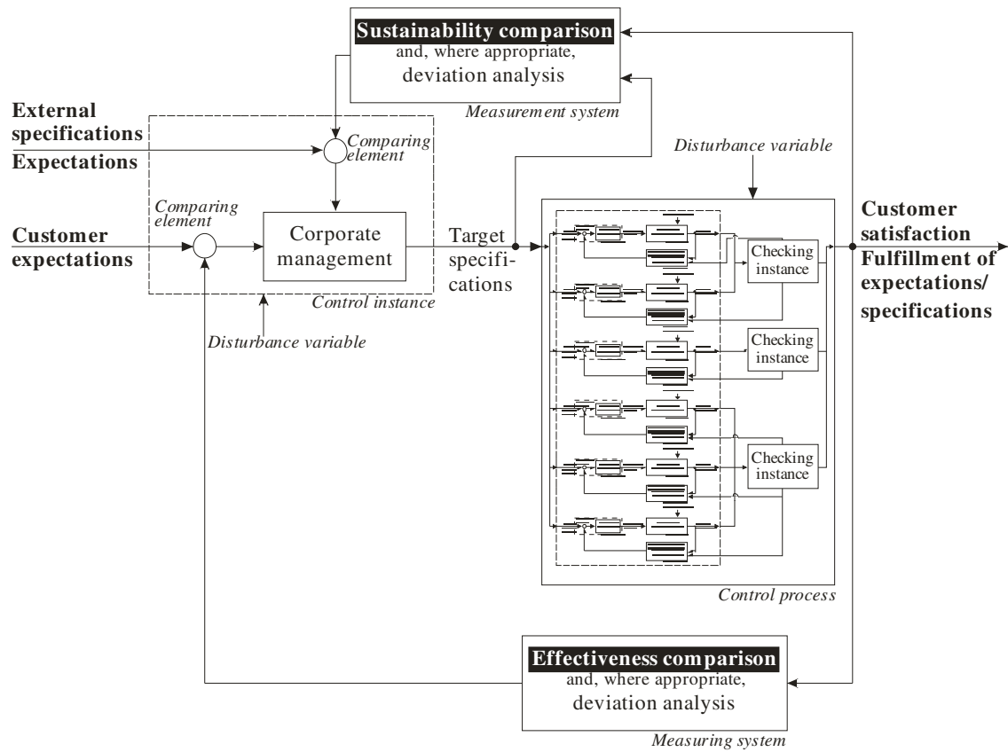
Figure 2: Sustainable Control Loop Architecture
